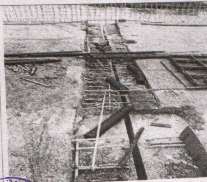
Location of expansion and contraction joints
